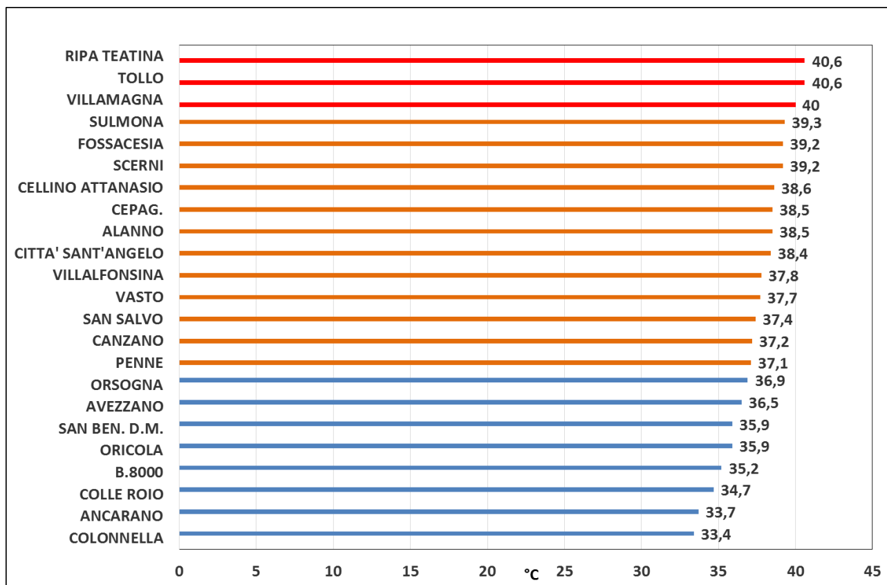
Fig. 8 Temperature massime assolute
